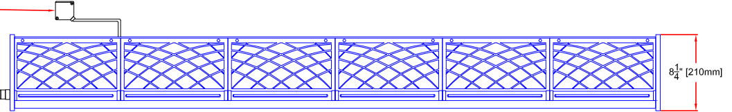
TOP VIEW
