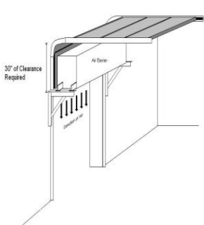
Standard Lift Door (SL)
