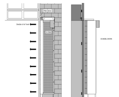
Vertical Air Barrier Installation
